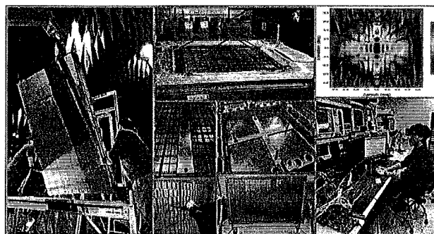
Figure 3 SAR-XL EM panel undergoing Manufacturing, Assembly and RF Range and Electronics Testing
