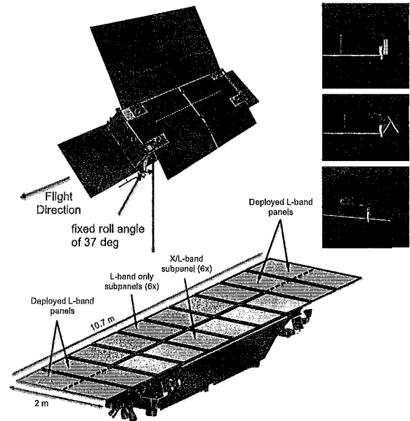
Figure 6 SAR-XL Antenna Configuration with 10 panels
