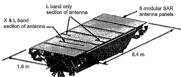
Figure 2 Spacecraft Configuration using 6 SAR-XL Panels (image courtesy of SSTL)
