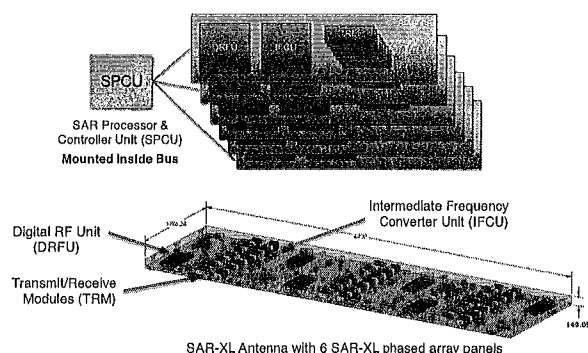
Figure 1 SAR-XL Payload Architecture & Configuration
