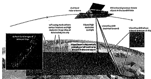
Figure 5 SAR-XL Advanced Maritime Surveillance Mode providing Wide Swath and High Resolution Imaging of Detected Objects
