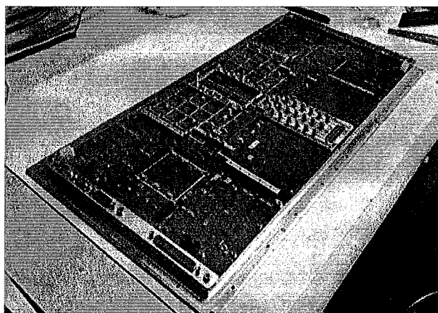
Figure 4 EM DRFU with the Prime Board on One Side and the Redundant Board on the Other Side
